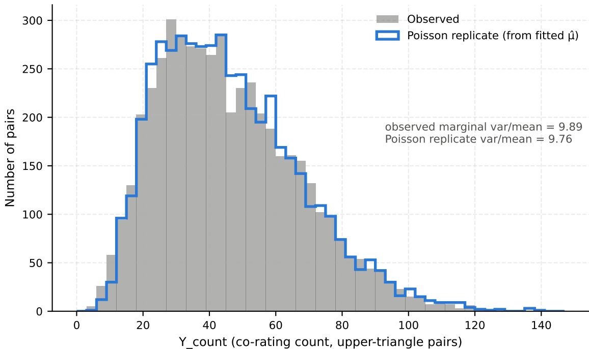
MovieLens Y_count vs plug-in Poisson replicate (k=5 fit) Marginal var/mean \approx 9.9 is reproduced by latent heterogeneity in \hat{\mu}
