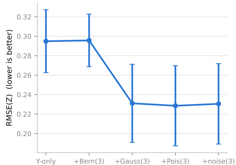
Attribute-addition ablation (per-column, 3 seeds)
