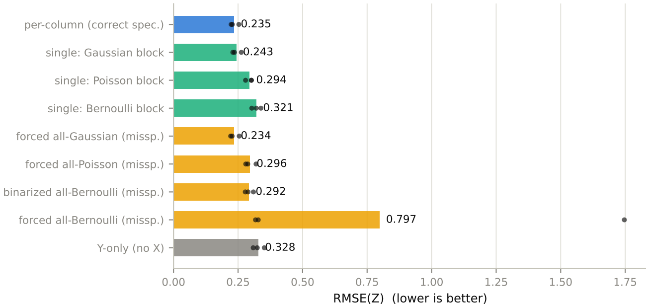
Mixed-X synthetic: RMSE(Z) by condition (3 seeds, Procrustes)
