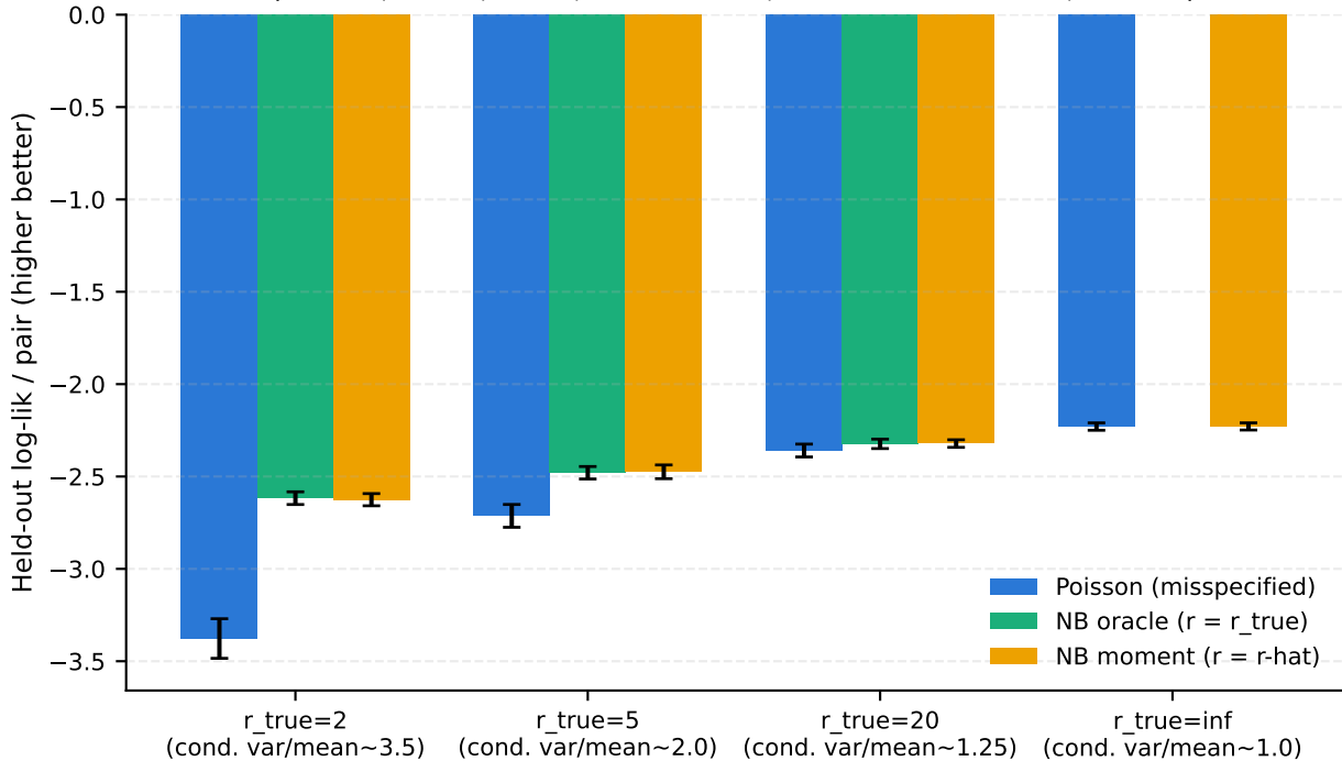
Held-out predictive likelihood vs overdispersion strength ( n=100 , d=15 , k^*=3 , X=\text{Bernoulli} , strict held-out 20%, 5 trials)
