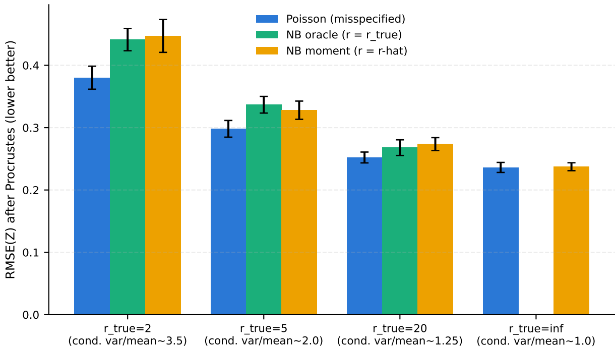
Latent structure recovery vs overdispersion strength ( n=100 , d=15 , k^*=3 , X=\text{Bernoulli} , strict held-out 20%, 5 trials)
