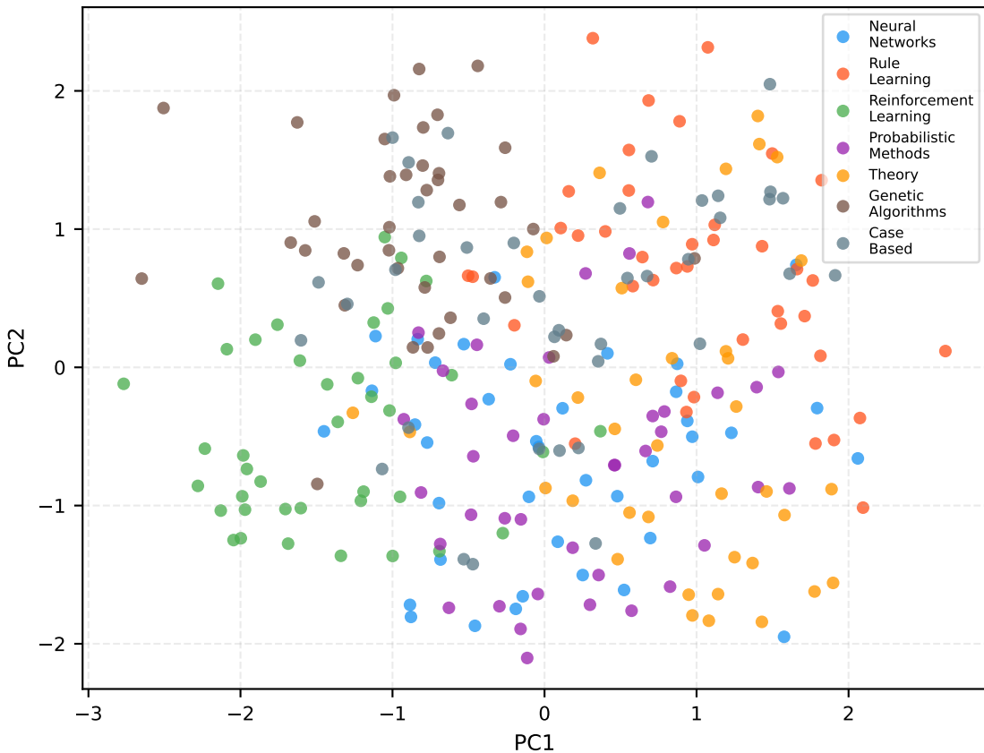
Cora balanced_degree — Z (k=3, split=1, model=1) test_AP=0.5402 NMI=0.3087
