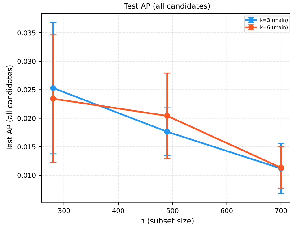
Cora scaling held-out link prediction — prediction metrics vs n (main: n=280/490/700, mean±std over 3 splits; stress: n=980, single split, no std)
