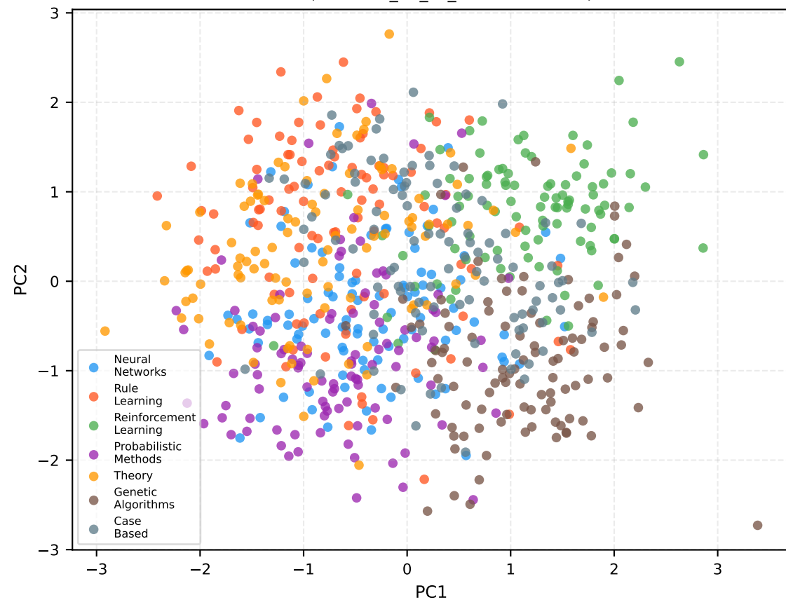
k=3 (best test_AP_all_candidates trial)
