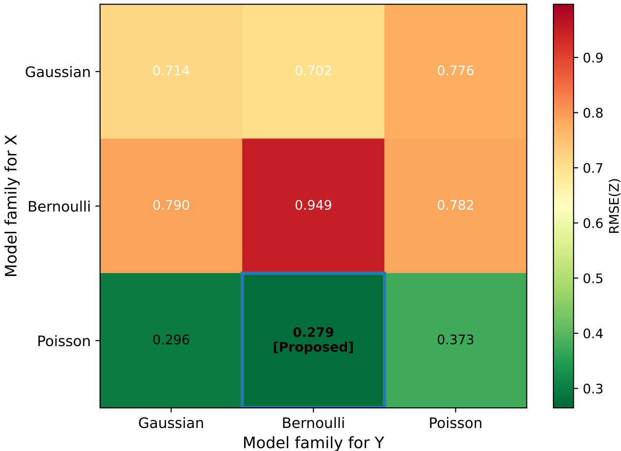
Fig 4: RMSE(Z) Mismatch Heatmap True data: X=Poisson, Y=Bernoulli (n=150, d=15, k=3)
