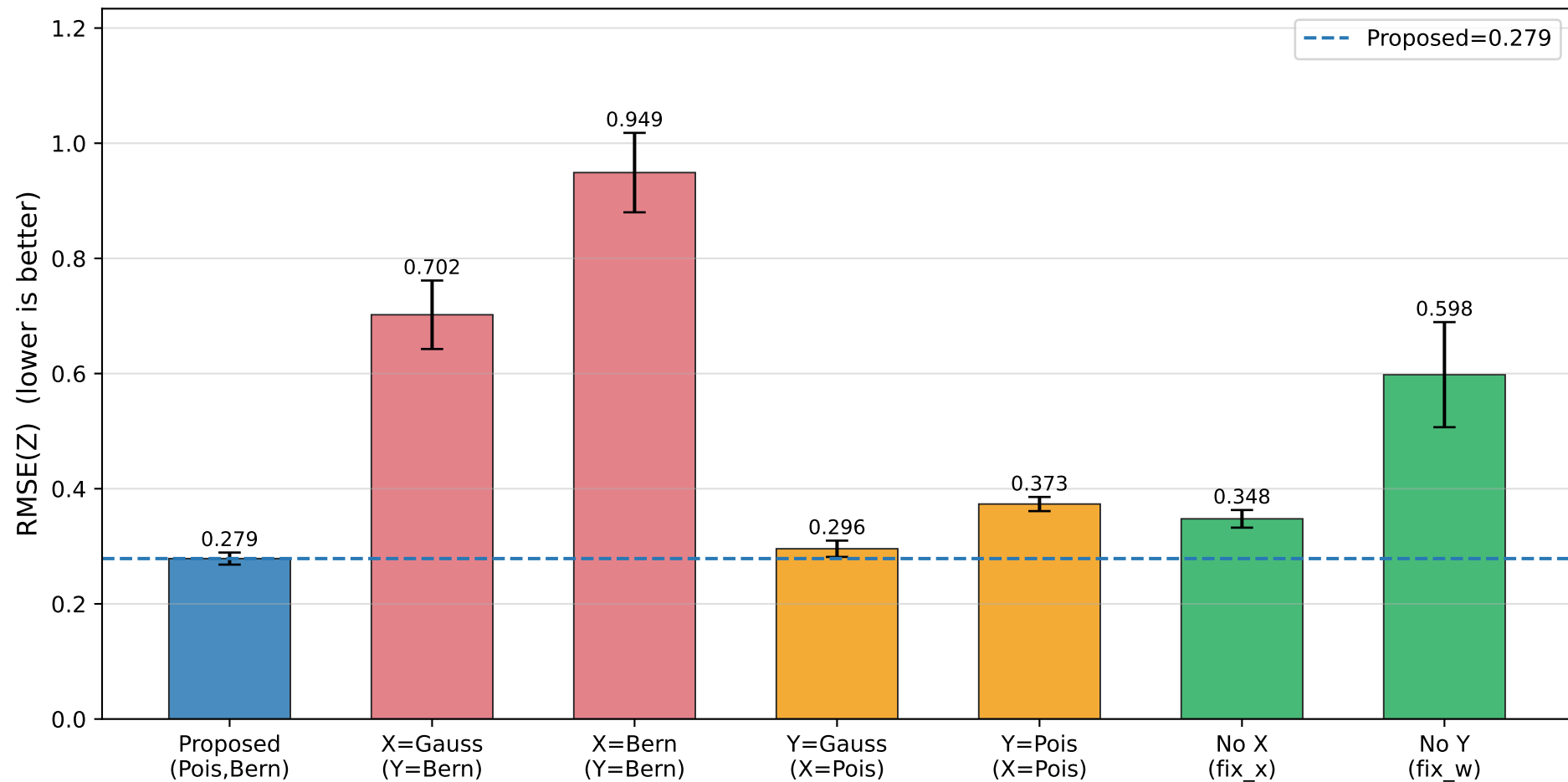
Scenario A: RMSE(Z) Comparison True: X=Poisson, Y=Bernoulli (n=150, d=15, k=3, 10 trials)
