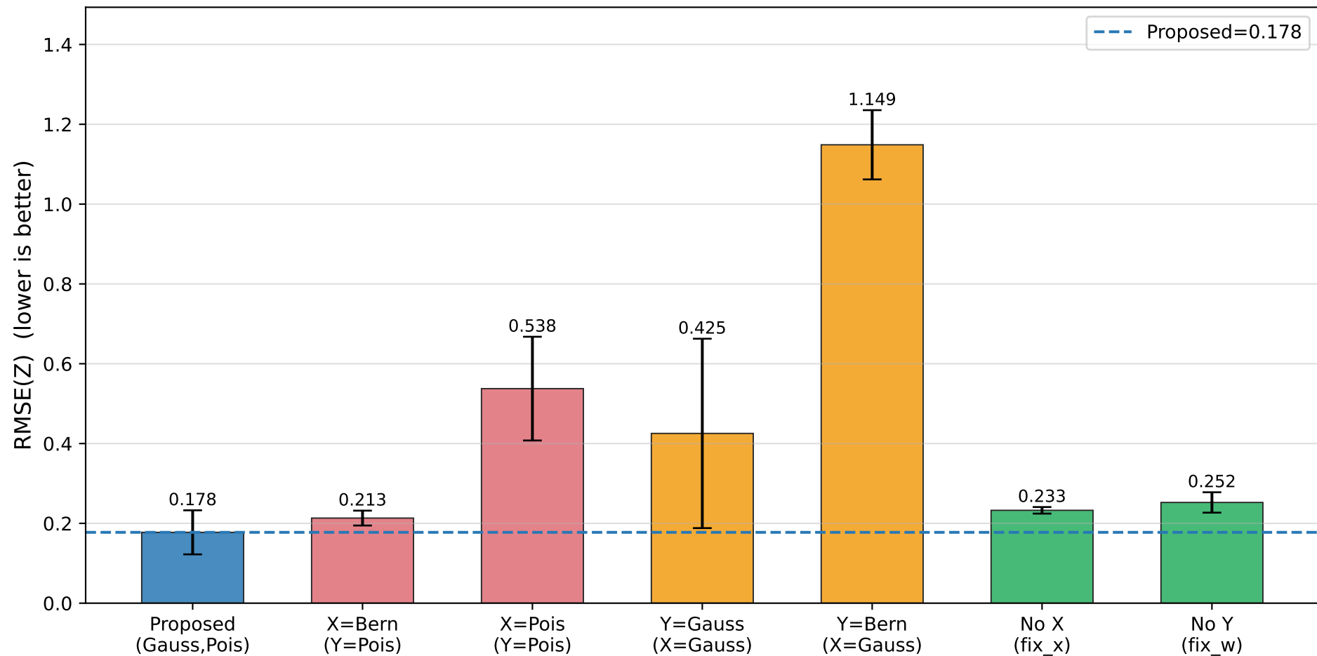
Scenario B: RMSE(Z) Comparison True: X=Gaussian, Y=Poisson (n=150, d=15, k=3, 10 trials)
