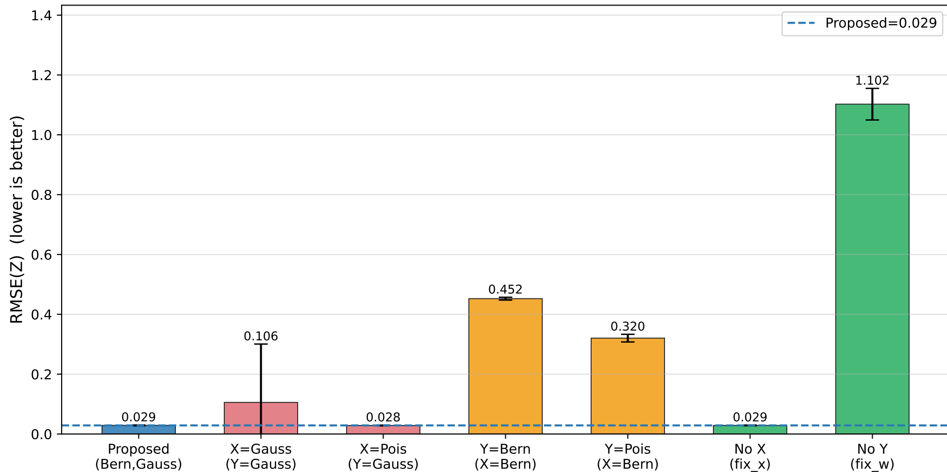
Scenario C: RMSE(Z) Comparison True: X=Bernoulli, Y=Gaussian (n=150, d=15, k=3, 10 trials)
