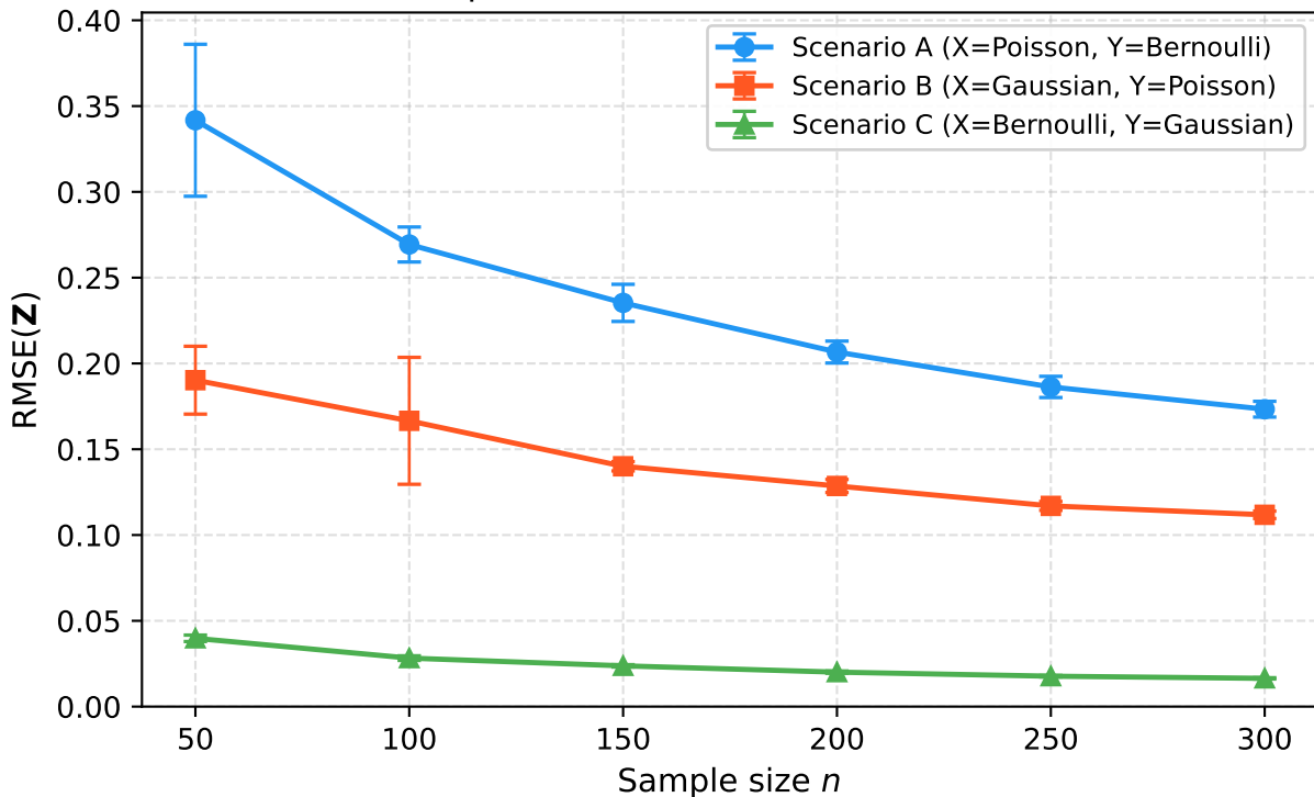
n-sweep: RMSE( \mathbf{Z} ) vs. Sample Size (fixed implementation, 10 trials, d = 15 , k^* = 3 )
