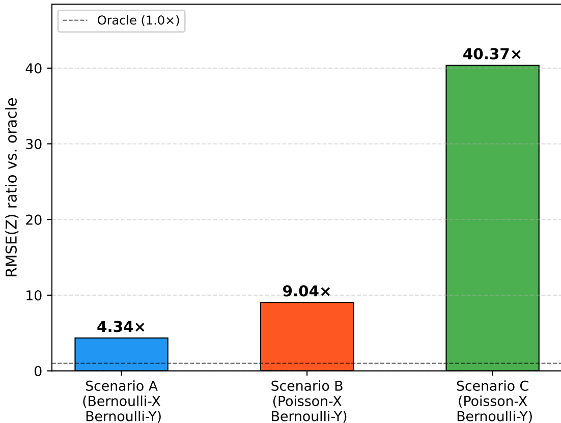
Distribution Misspecification Impact (max ratio in 3 \times 3 grid, ablation excluded, fixed implementation)
