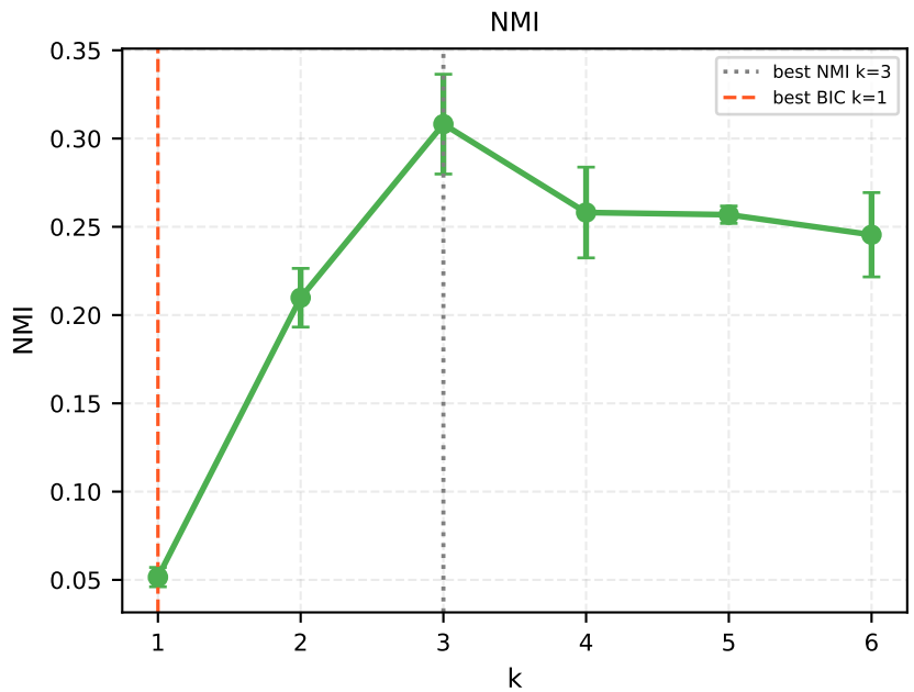
Cora balanced_degree — Metrics vs k (mean \pm std) (n=280, d=50, X=Bern, Y=Bern, 3 trials/k)
