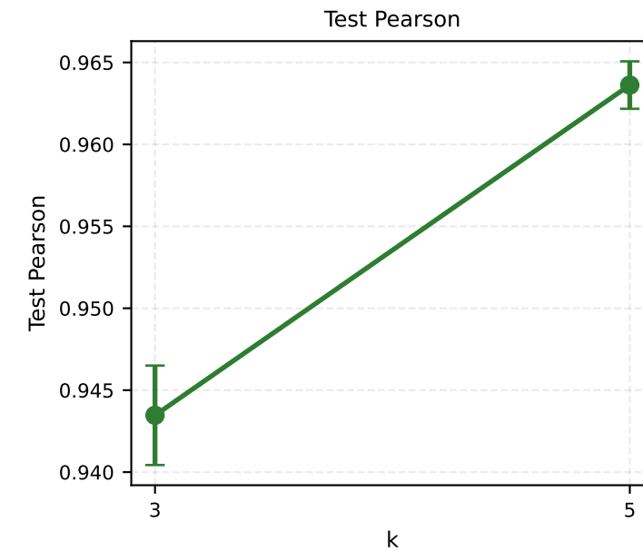
MovieLens held-out count regression — Metrics vs k (MASKED EVALUATION: trained on all pairs, eval split into train/test) (n=100, d=19, X=Bern, Y=Pois, 3 splits × 2 models/k)
