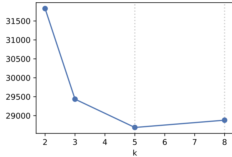
BIC vs k
