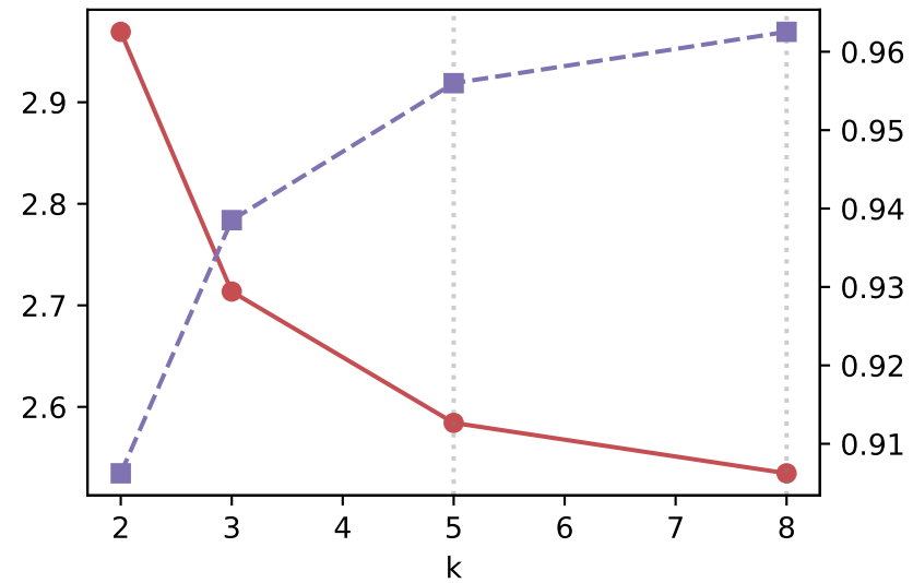
Y reconstruction vs k (Poisson Y)
