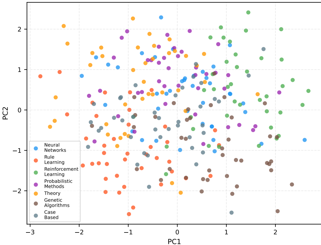
Cora balanced_degree — Z (k=6, split=1, model=1) test_AP=0.5632 NMI=0.2154
