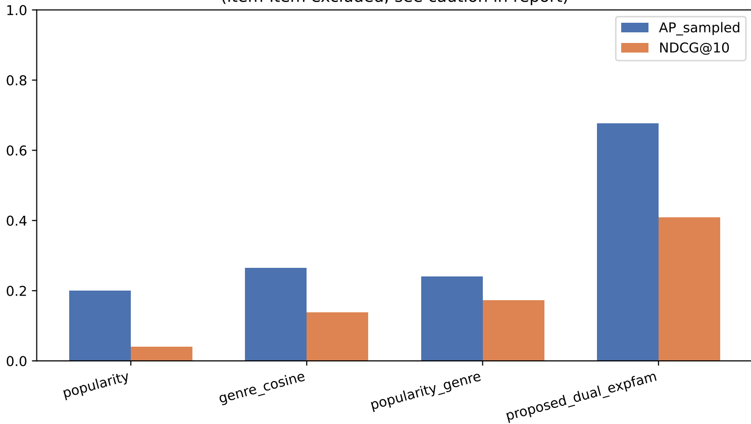
Lift link prediction: proposed vs. simple baselines (item-item excluded; see caution in report)
