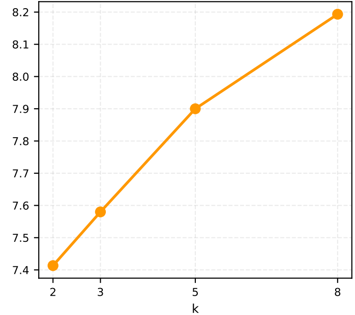
runtime (s)
