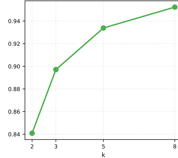
high_colike AP
