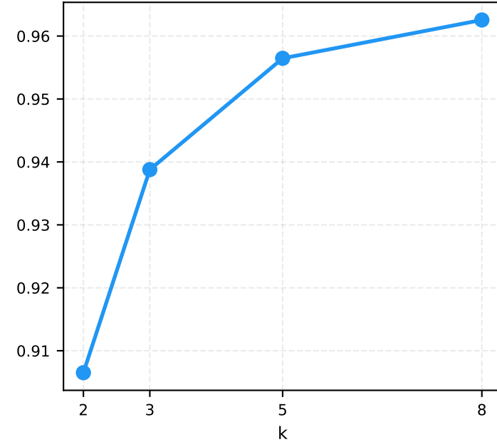
Pearson(Y,Y_hat)
