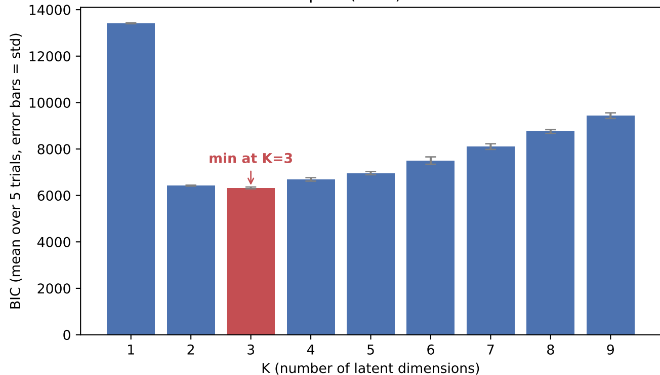
Wine pilot (fixed): BIC vs K
