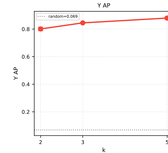
MovieLens Bernoulli t=80 — In-sample Metrics vs k (mean+/-std) (n=100, d=19, X=Bern, Y=Bern, density=0.0687, 3 trials/k)
