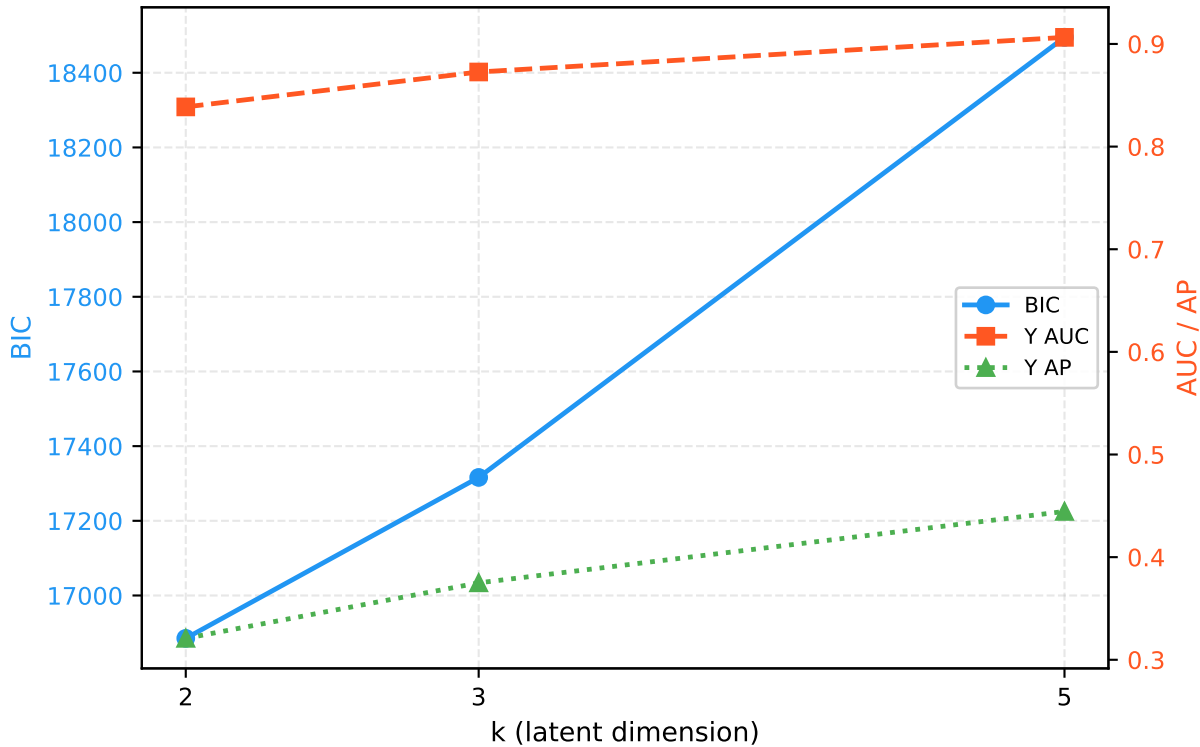
Cora Subset Pilot: BIC and Y-Reconstruction vs. k ( n=300 , d=50 , X=\text{Bernoulli} , Y=\text{Bernoulli} )
