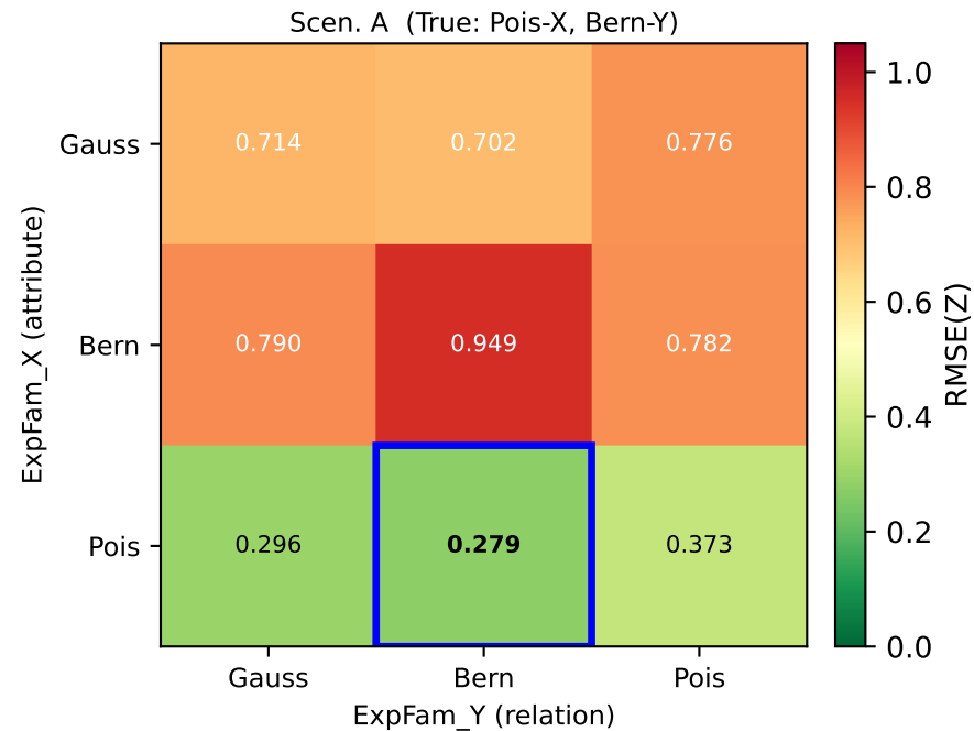
Distribution mismatch effect on RMSE(Z) [blue = correct specification]
