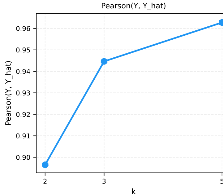
MovieLens Poisson Y pilot — Metrics vs k (mean \pm std) (n=100, d=19, X=Bern, Y=Pois, 3 trials/k)
