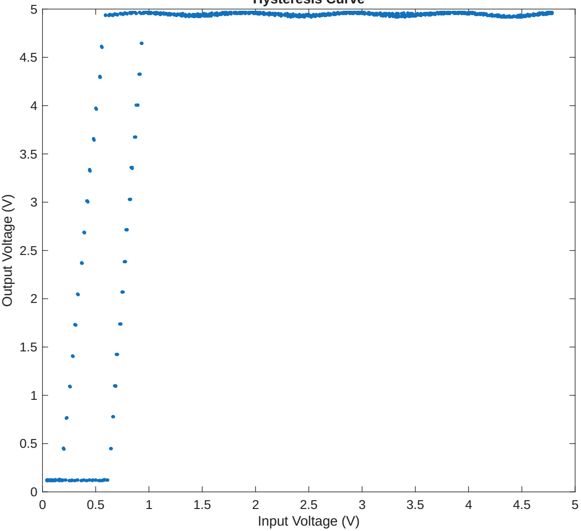
Hysteresis Curve
