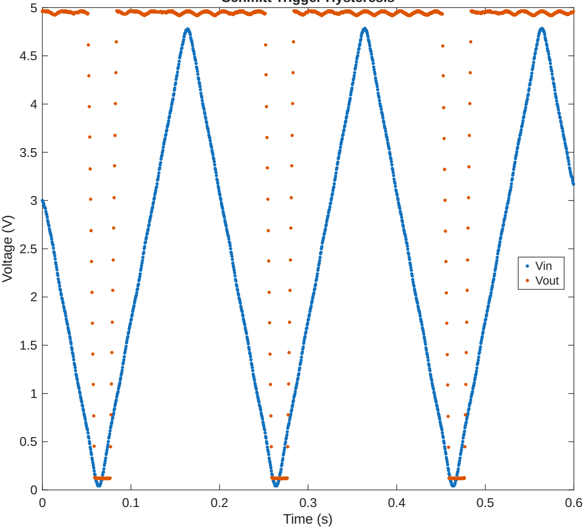
Schmitt Trigger Hysteresis
