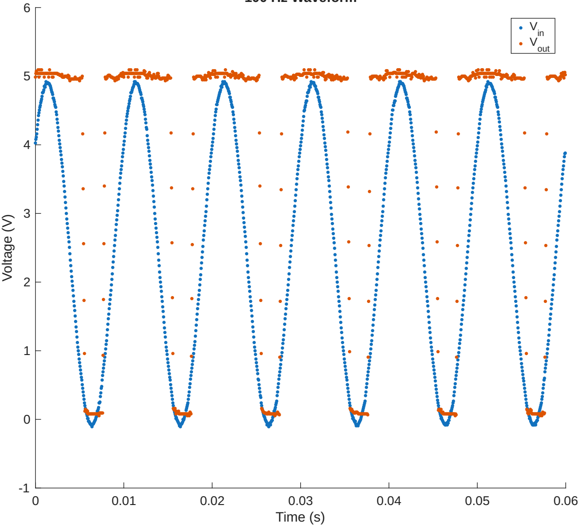
100 Hz Waveform
