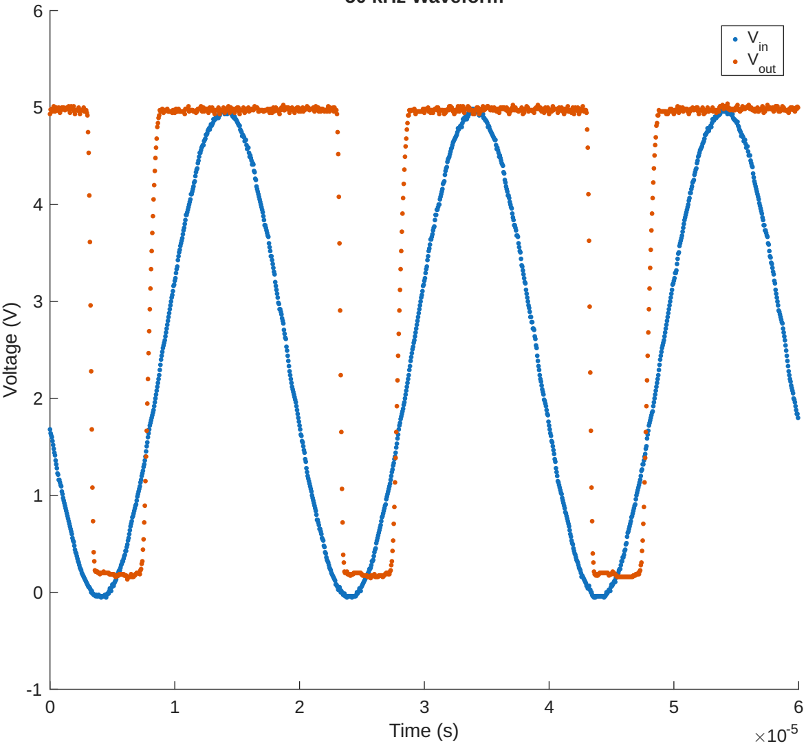
50 kHz Waveform
