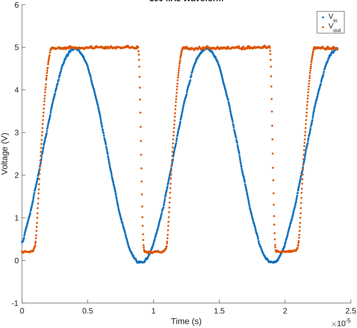
100 kHz Waveform
