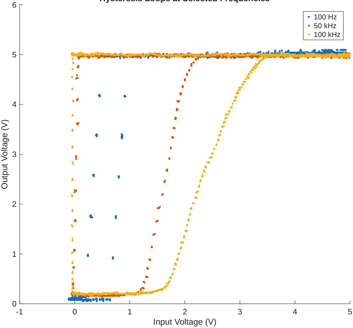
Hysteresis Loops at Selected Frequencies
