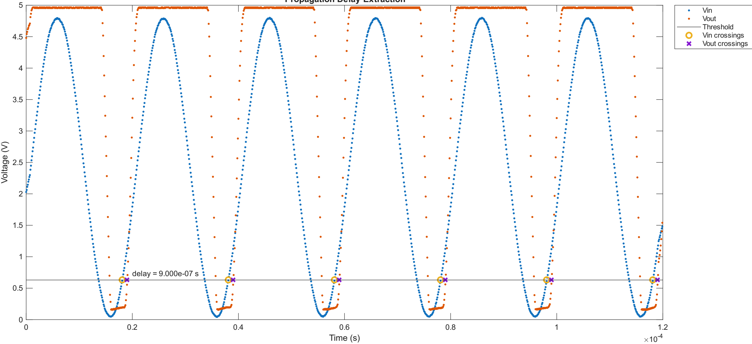
Propagation Delay Extraction
