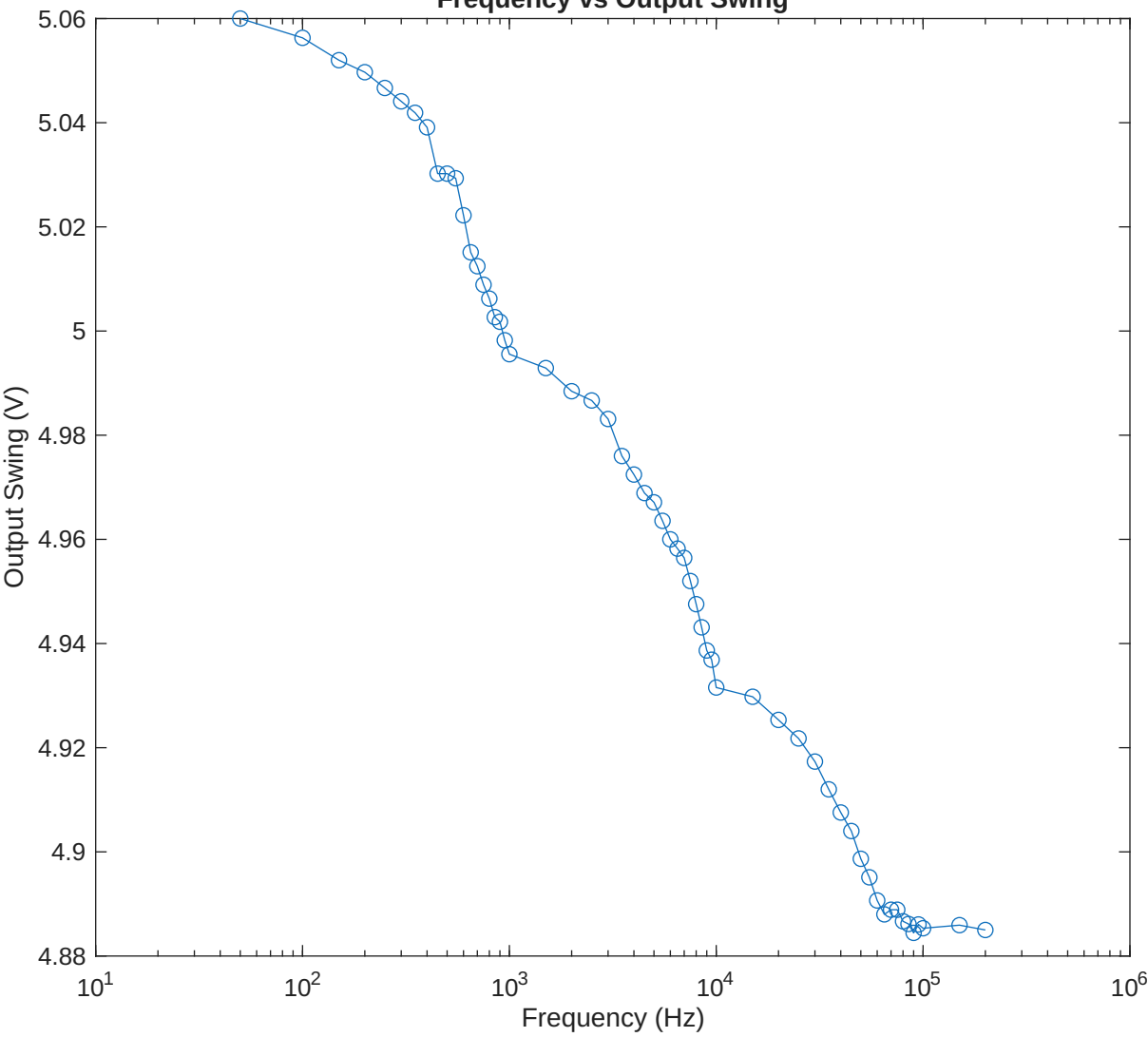
Frequency vs Output Swing
