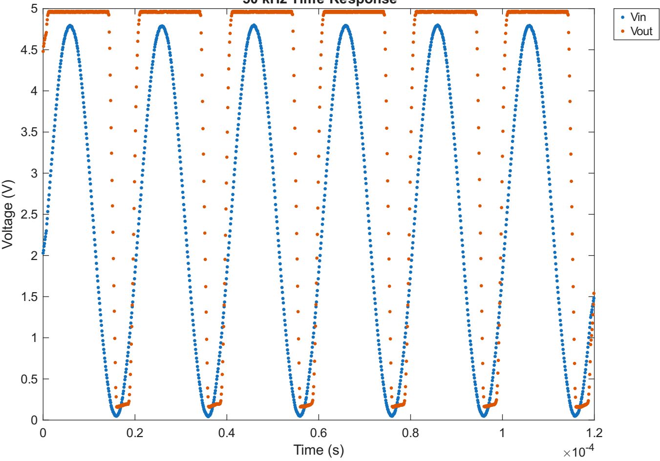
50 kHz Time Response
