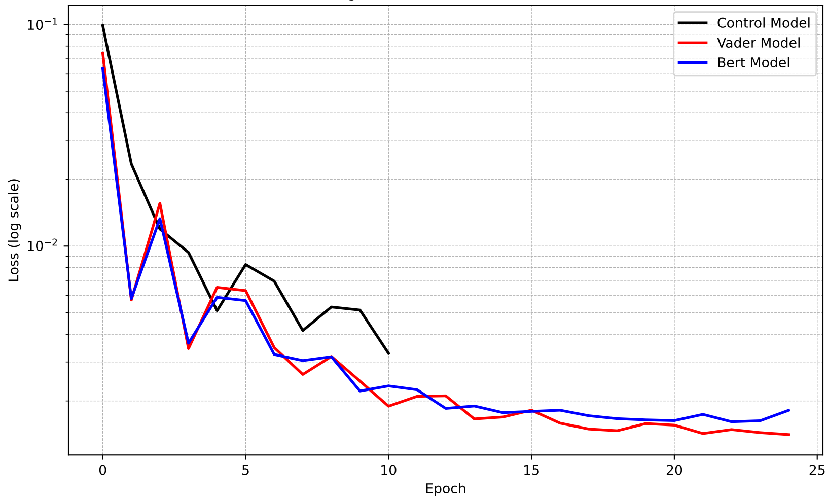
Training Loss of Different RNN Models
