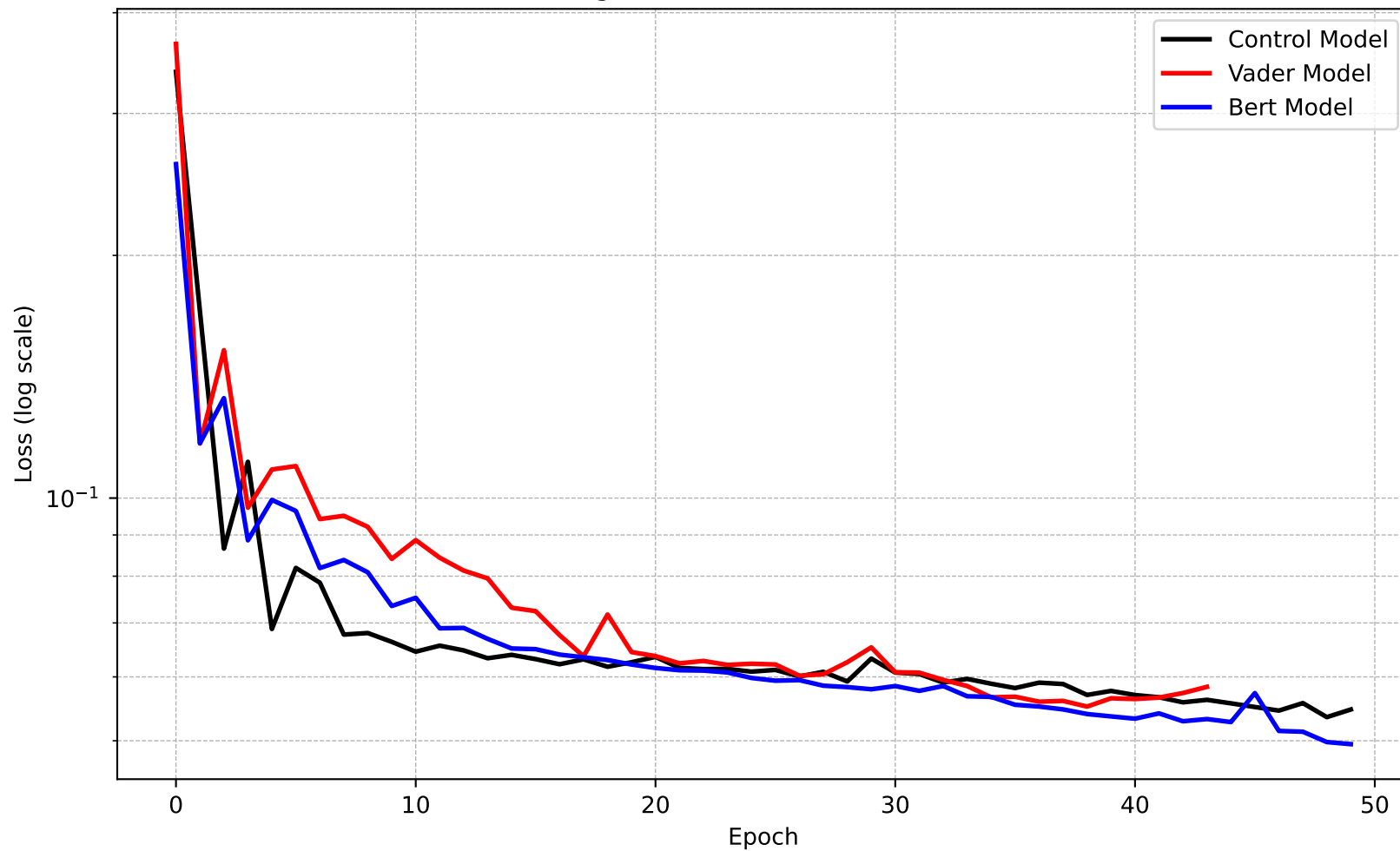
Training Loss of Different RNN Models
