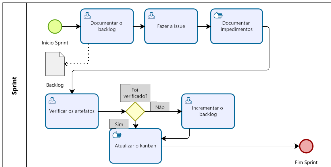
Figura 7 – BPMN Sprint
