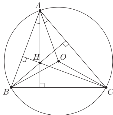
Figure 1.1D. The orthocenter and circumcenter. See Section 0.2 if you are not familiar with these.
