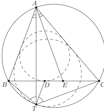
Figure 4.8B. Segments \overline{AT} and \overline{AE} are isogonal in \triangle ABC , while segments \overline{TD} and \overline{TA} are isogonal in \triangle TBC .
