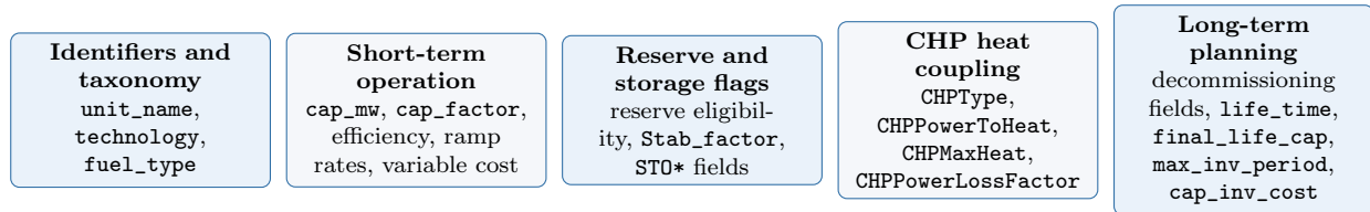
Figure 5: The file mixes identifiers, operational data, storage/reserve fields, CHP coupling terms, and planning trajectories.
