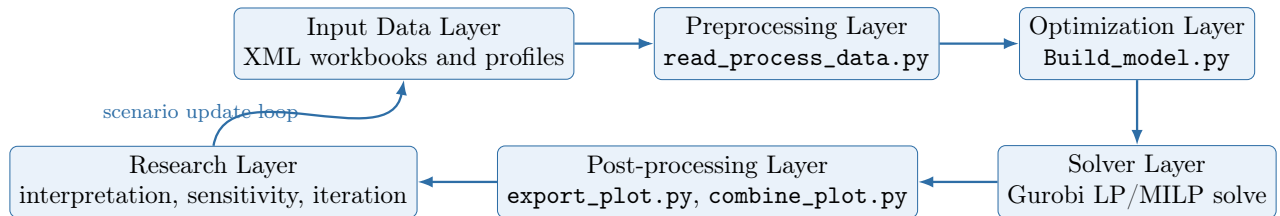
Figure 1: Layered architecture of H2RES from data engineering to research decisions.
