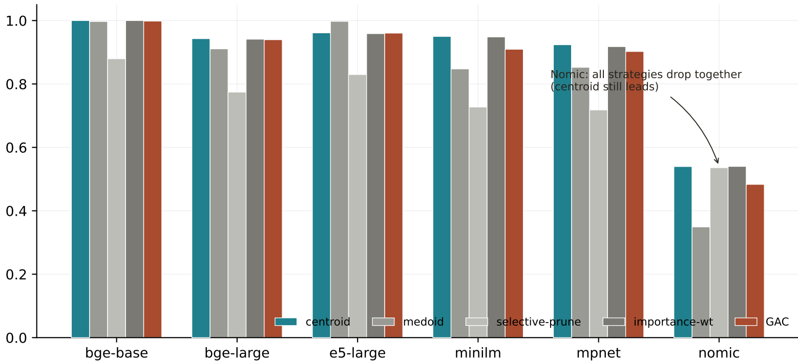
Identity accuracy (DRM-templated)
