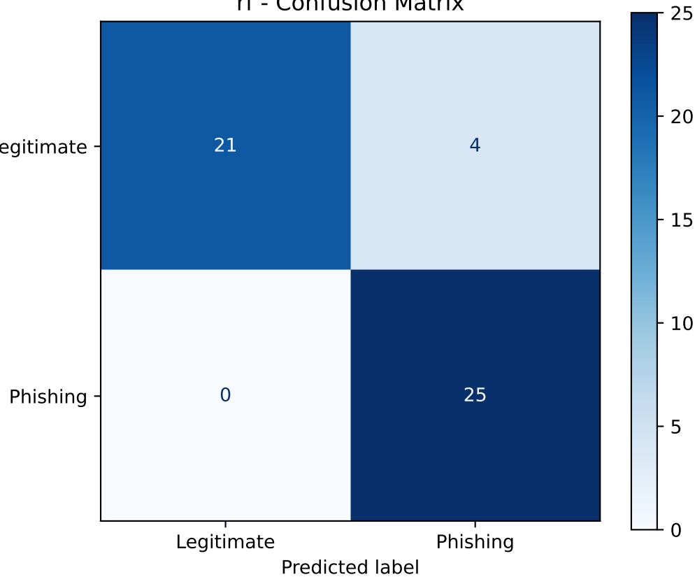
rf - Confusion Matrix
