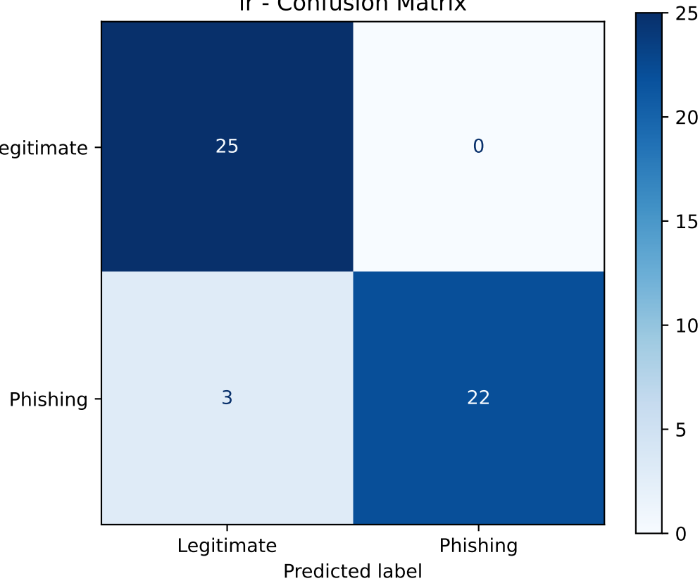
Ir - Confusion Matrix
