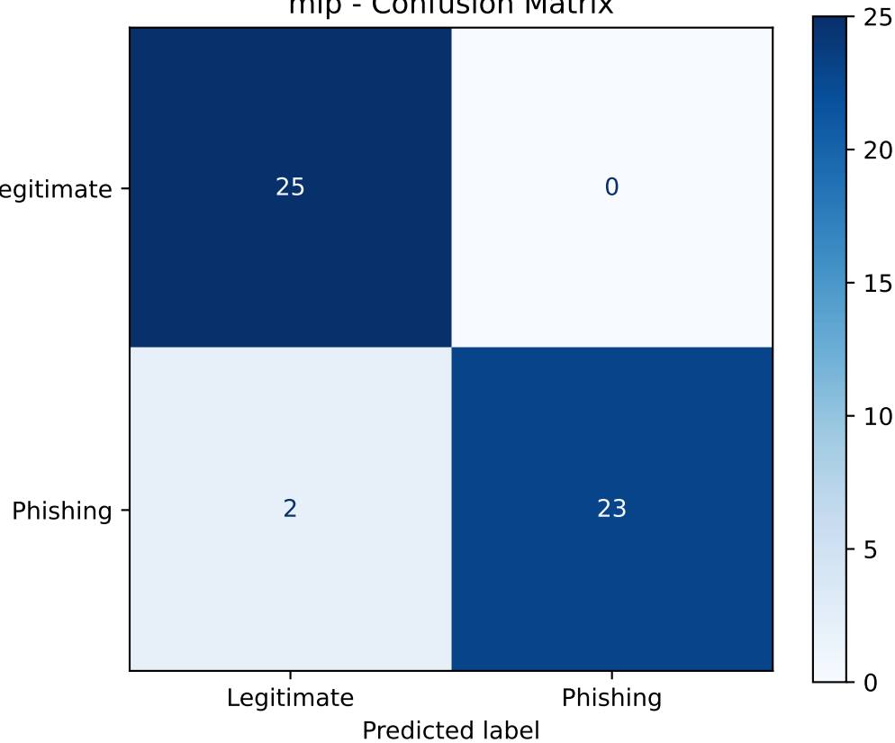
mlp - Confusion Matrix
