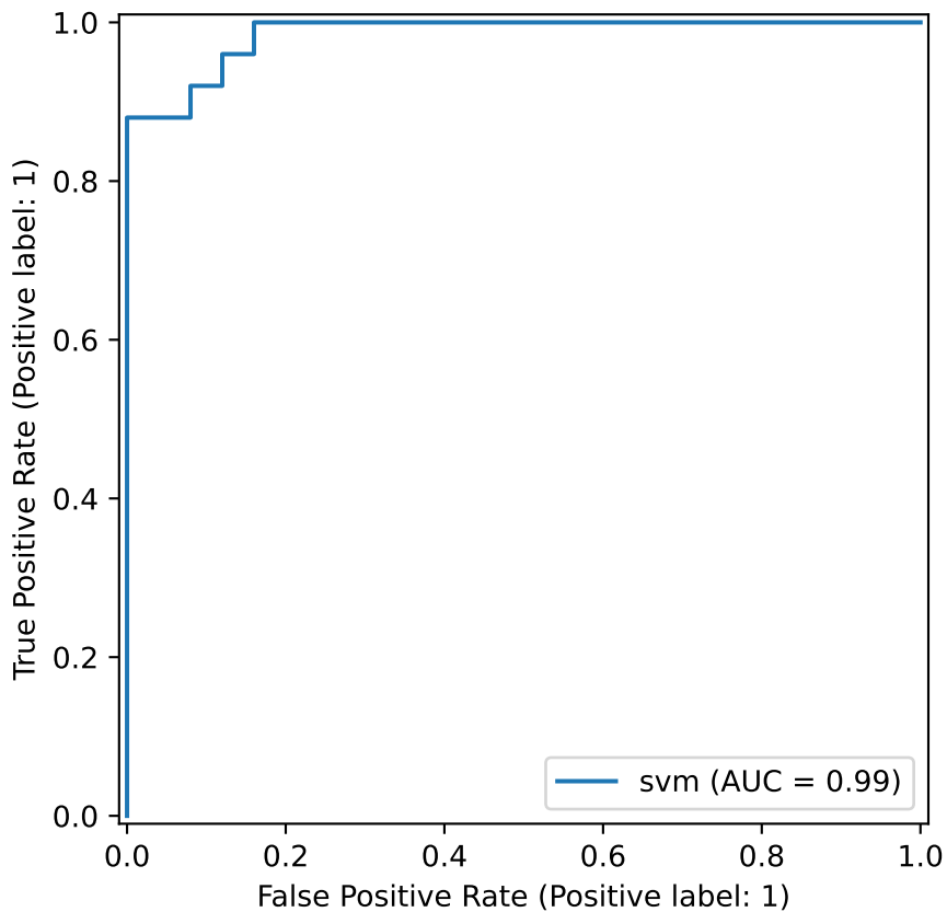
svm - ROC Curve
