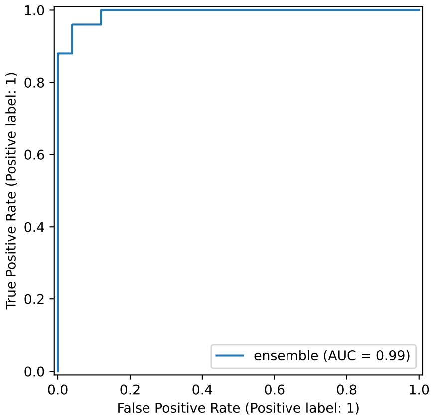
ensemble - ROC Curve
