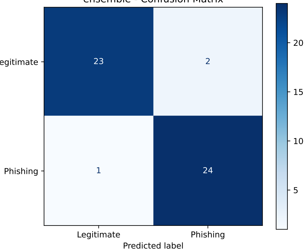
ensemble - Confusion Matrix
