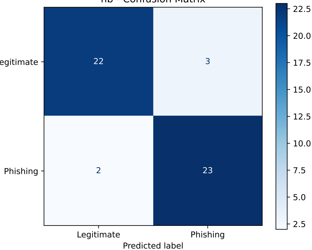
nb - Confusion Matrix
