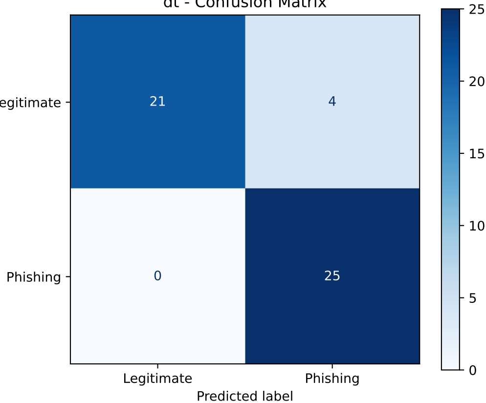
dt - Confusion Matrix
