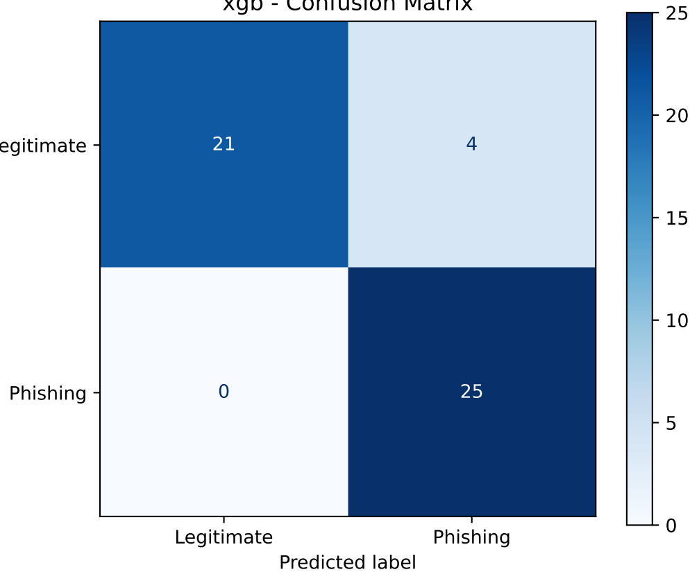
xgb - Confusion Matrix
