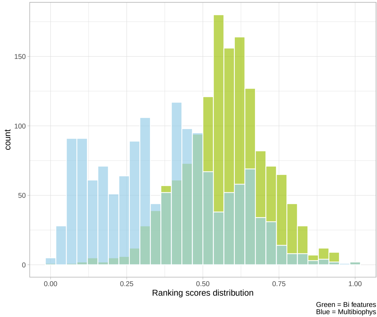
Bi-features vs. Multifeatures ranking scores distribution
