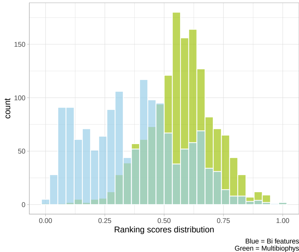
Bi-features vs. Multifeatures ranking scores distribution
