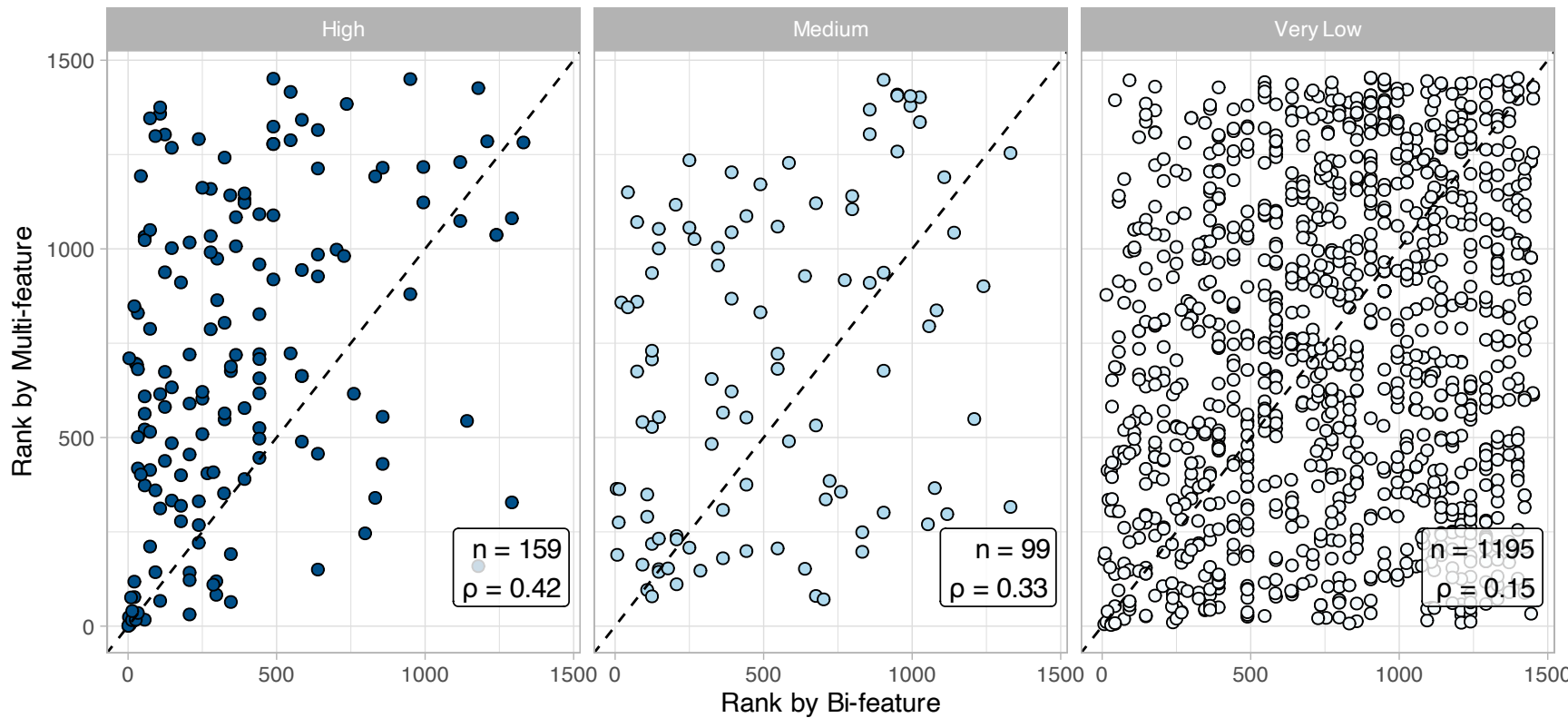
Faceted distribution of scoring metrics across evidence level
