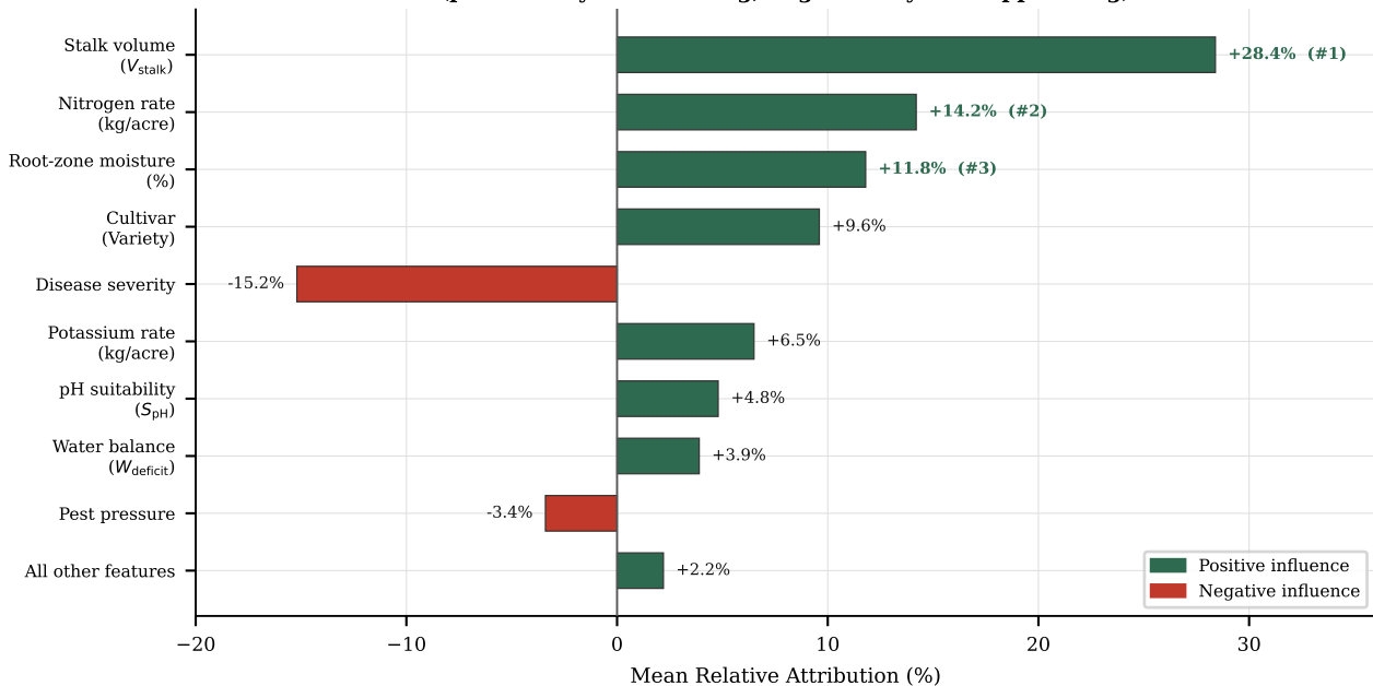
Fig. 6 - Global Feature Attribution via Integrated Gradients (positive = yield-boosting; negative = yield-suppressing)
