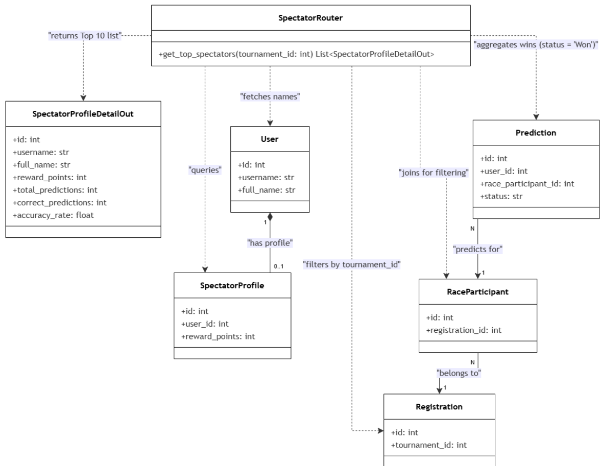
Figure 4.35: Top 10 Spectators Leaderboard Class Diagram
