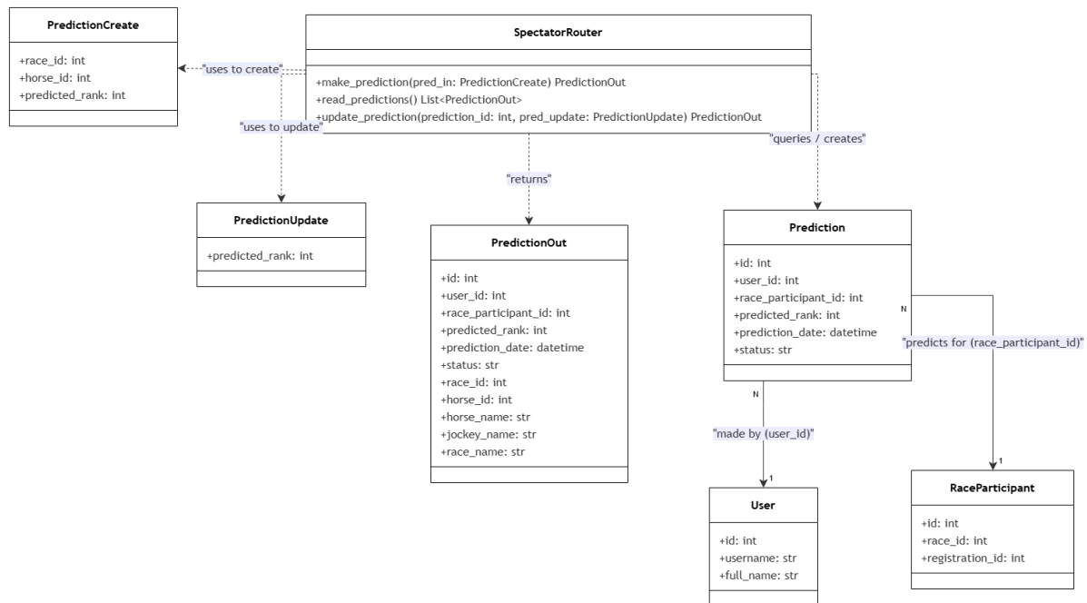
Figure 4.27: Spectator Prediction Class Diagram
