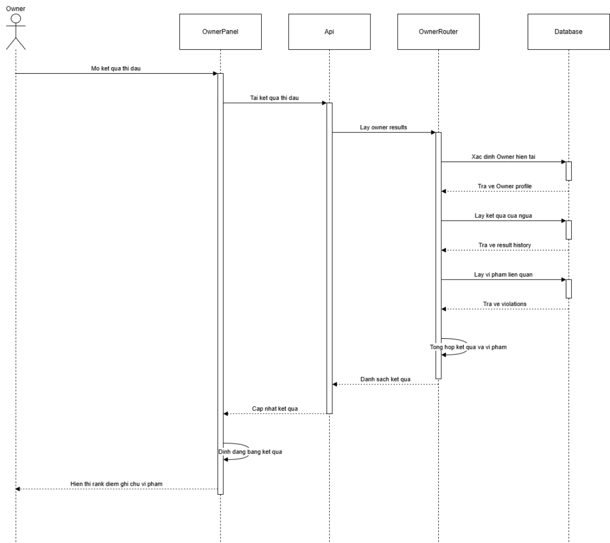
Figure 4.24: View Race Results Sequence Diagram
