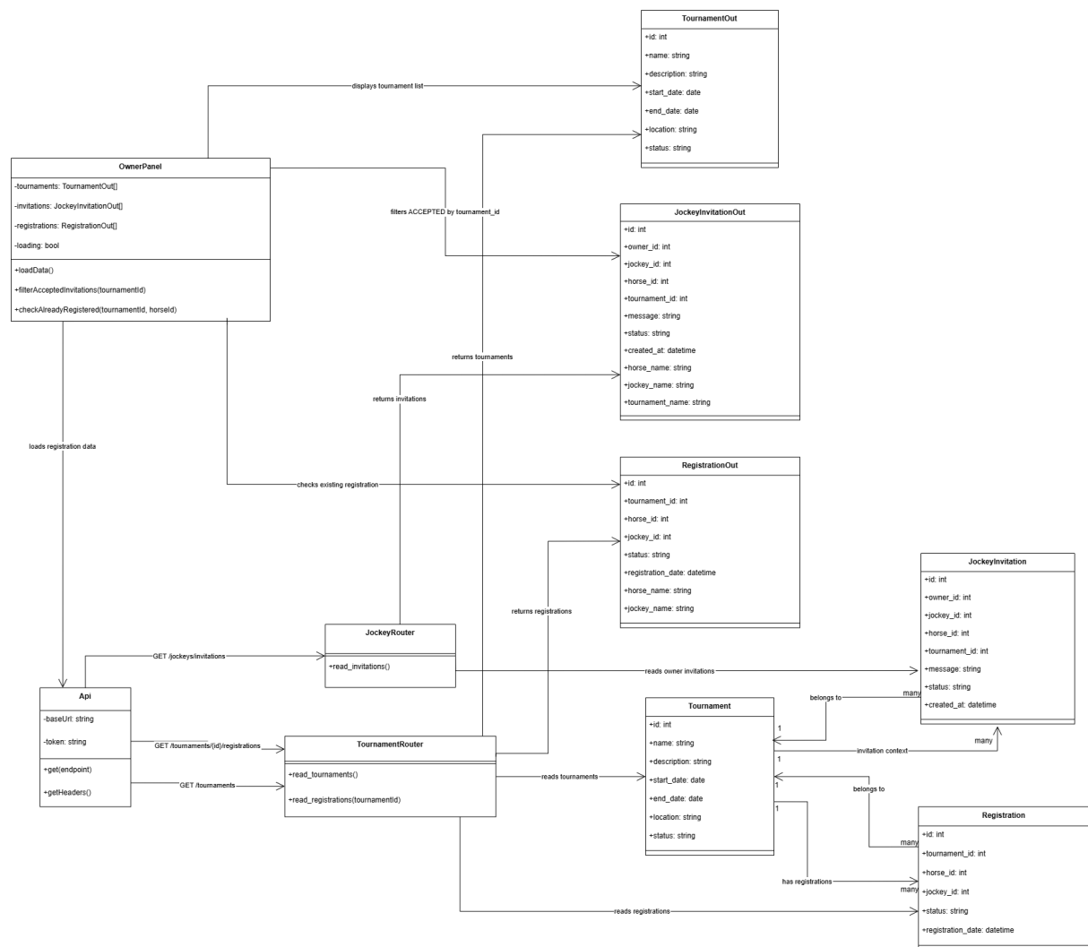
Figure 4.9: Tournament Registration Data Preparation Class Diagram
