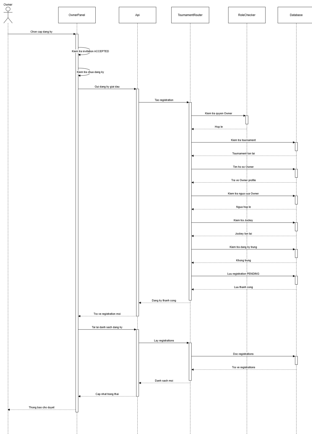
Figure 4.12: Submit Tournament Registration Sequence Diagram
