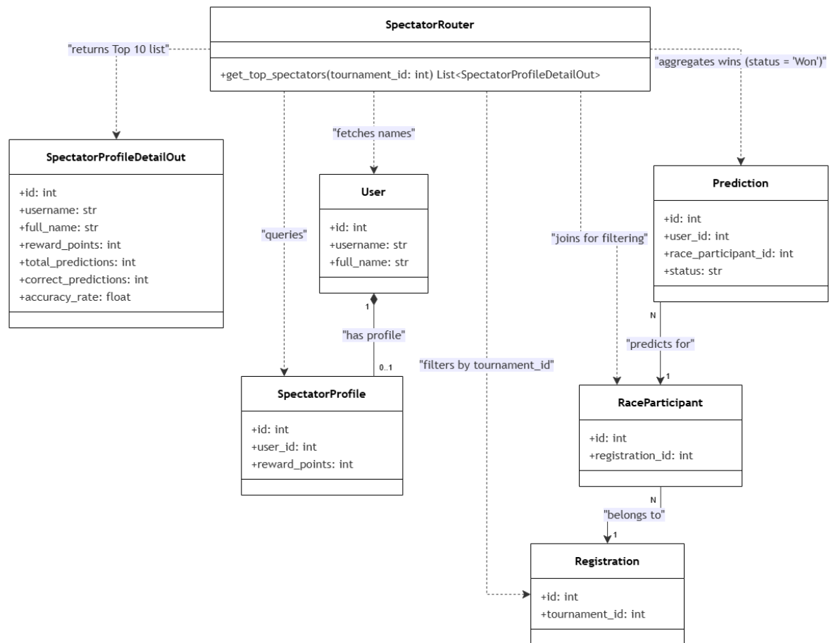
Figure 4.22: Top 10 Spectators Leaderboard Class Diagram
