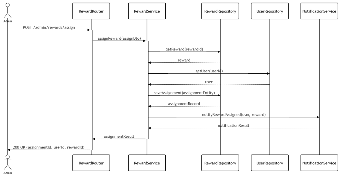
Figure 4.12: Admin Manage Rewards Sequence Diagram
