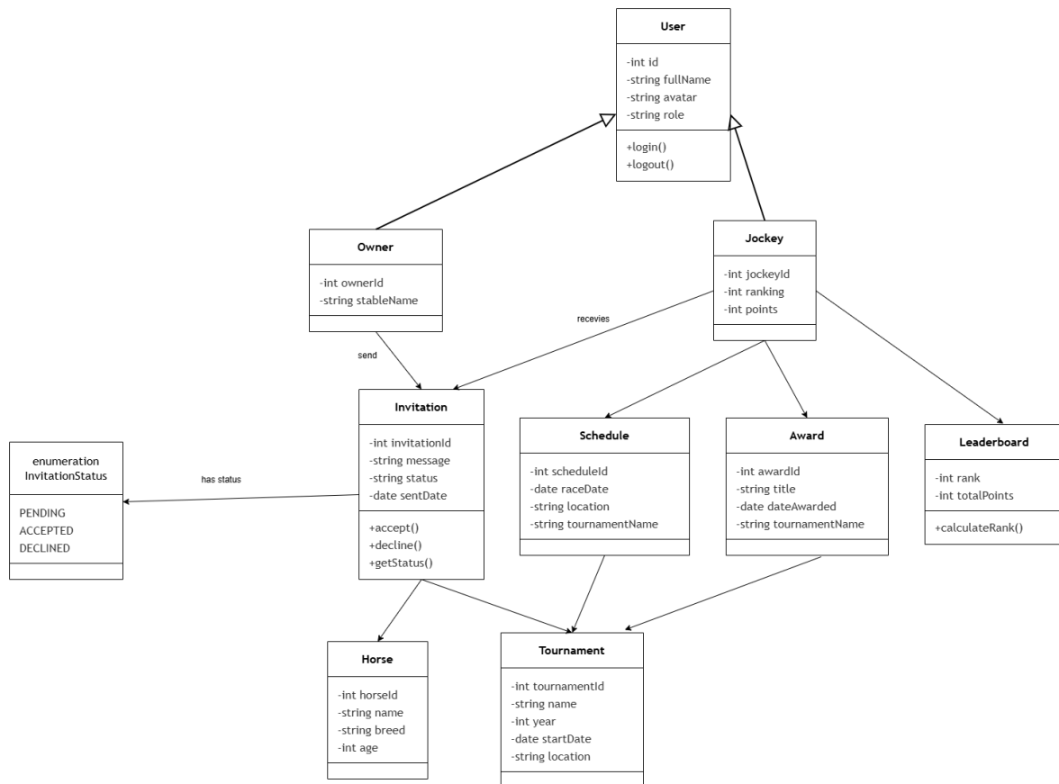
Figure 4.21: Jockey Dashboard Class Diagram
