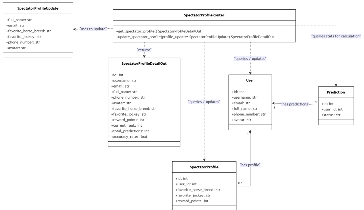
Figure 4.33: Spectator Personal Profile Class Diagram
