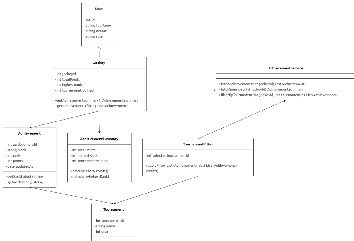
Figure 4.29: Achievements Class Diagram
