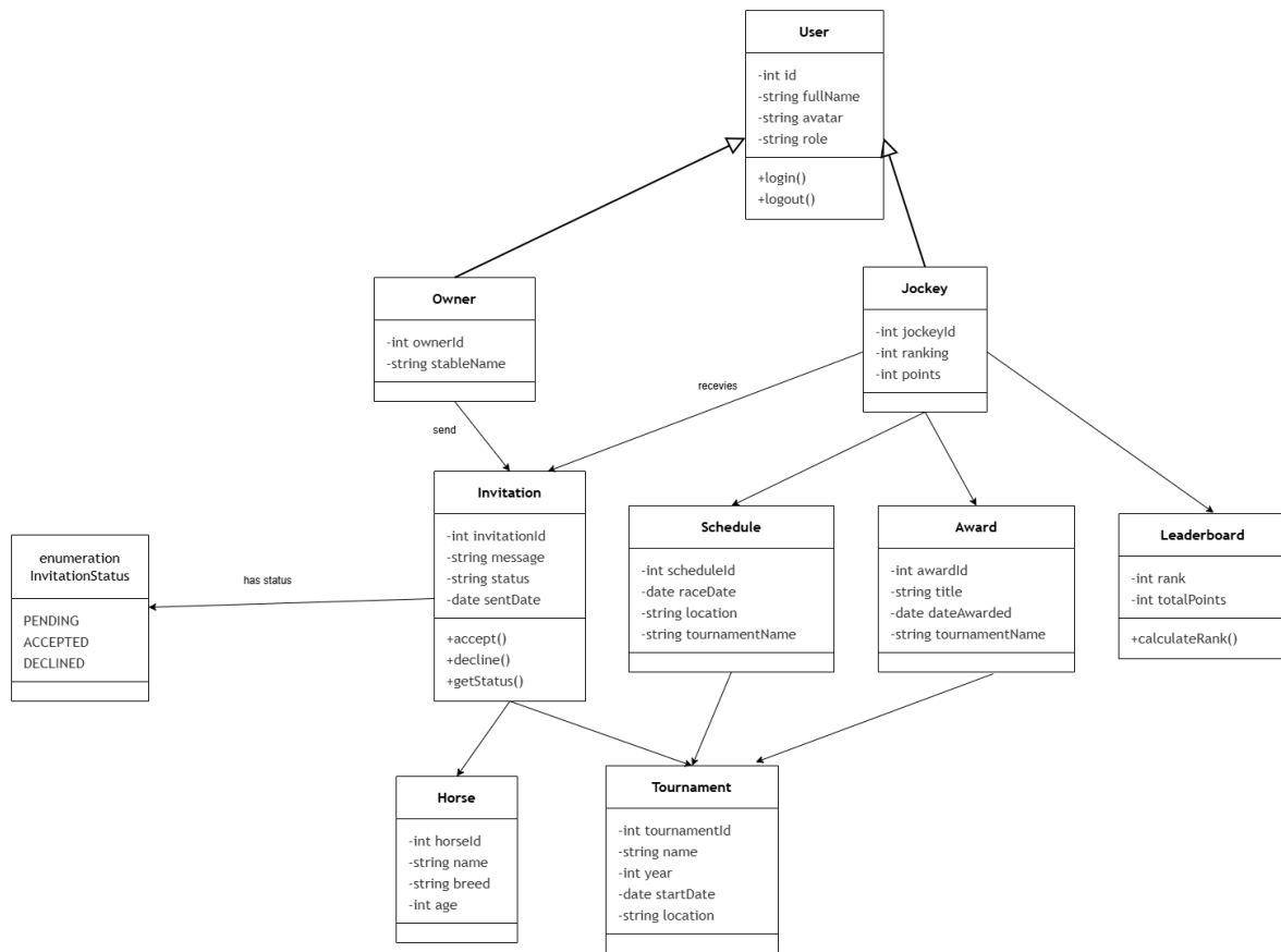
Figure 4.15: Jockey Dashboard Class Diagram
