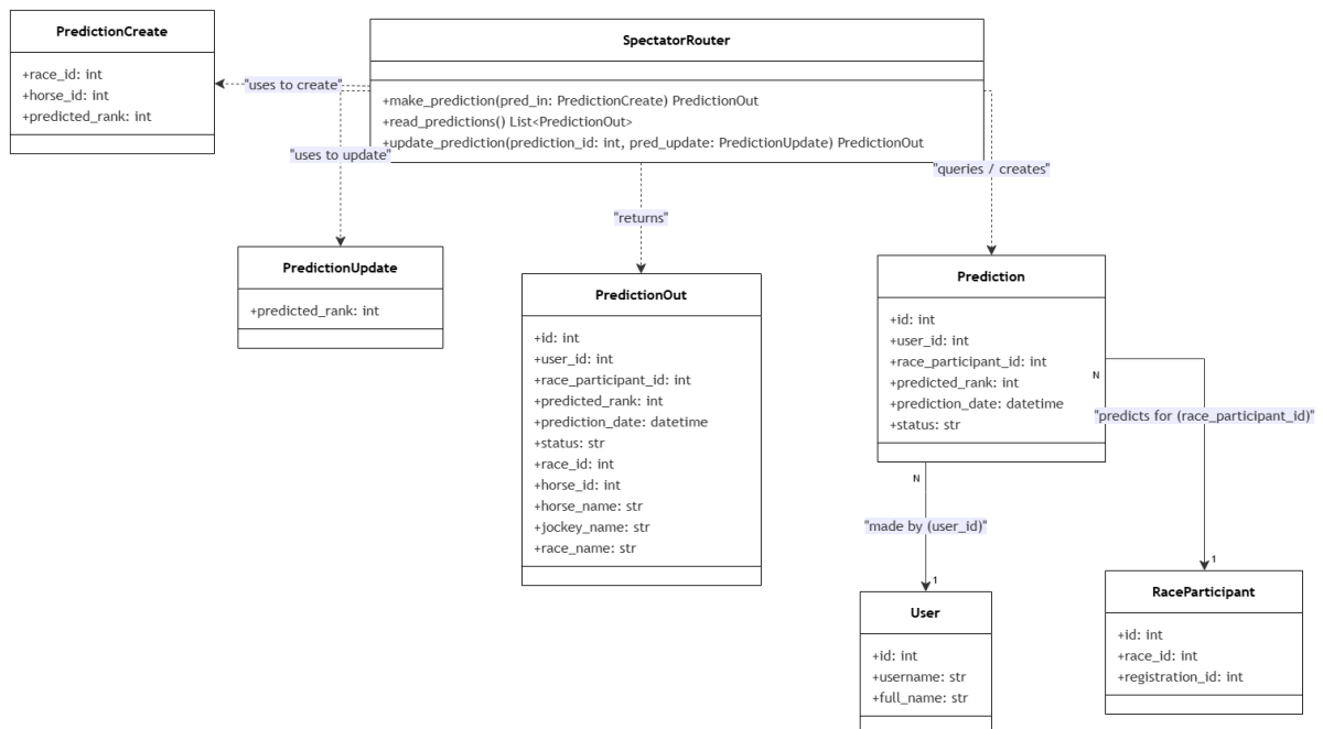
Figure 4.17: Spectator Prediction Class Diagram
