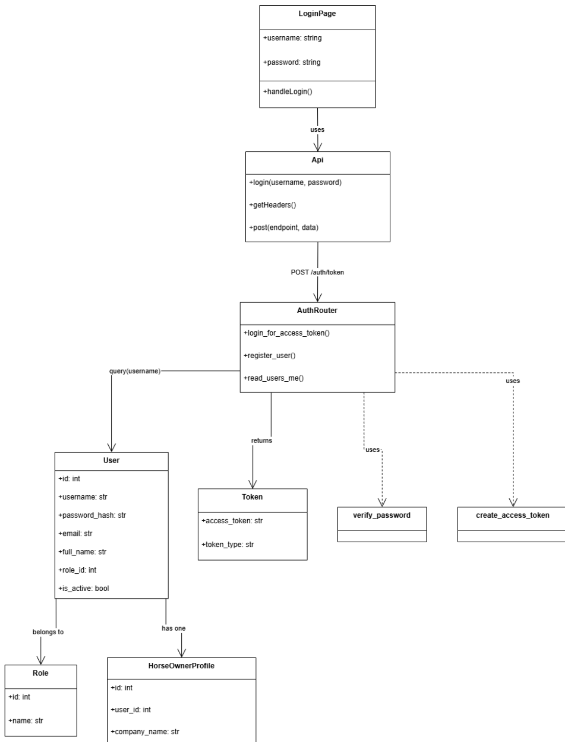
Figure 4.1: Login Class Diagram
